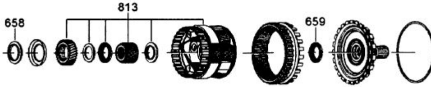
Rear Planetary Assembly
